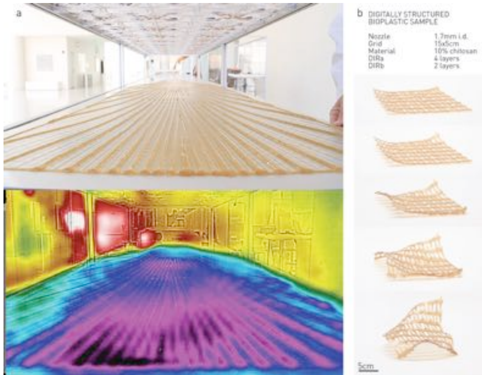
Figure 4: (a) Internal stresses generated by natural evaporation contribute to the shaping of each structural component. (b) 2D-to-3D shaping stages of an additively manufactured structured chitosan grid removed from the substrate at an intermediate state of curing (left to dry and form-found within 12 hours).
