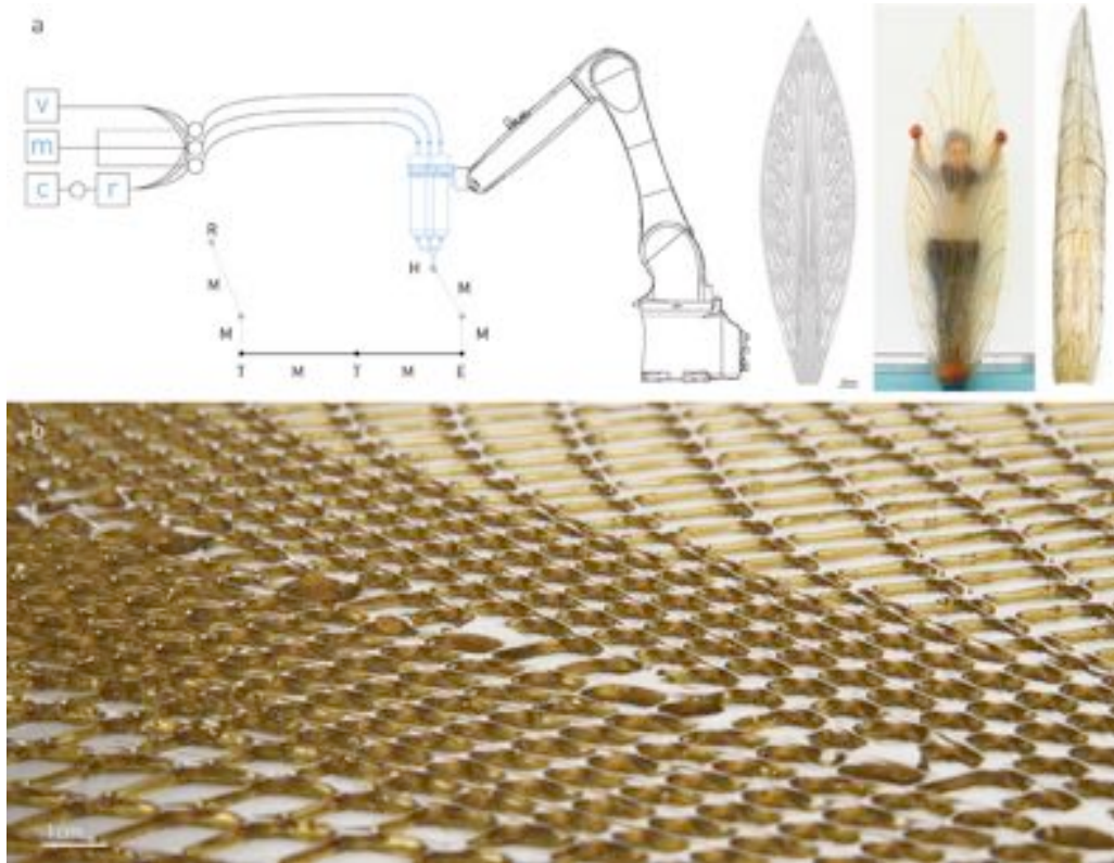
Figure 3: (a) Motion-extrusion instructions schema: a pneumatic assembly for material deposition is designed as a multi-chamber nozzle and attached to the end-effector of an existing positioning platform (Kuka KR AGILUS robotic arm; model KR 10 R1100 SIXX WP). (b) Close-up image of a hierarchically structured chitosan-based deposited construct.
